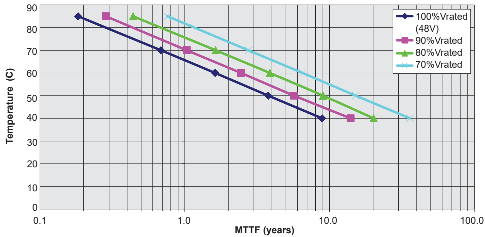
Expected Lifetime at Various Voltages SCM Series 48V Rated for Balanced Modules
