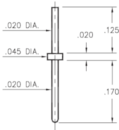
9081-0-00-XX-00-00-08-0 Solder mount in .024 mounting hole
